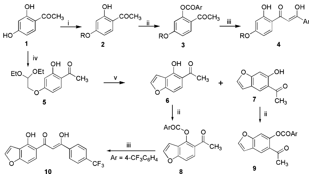
Scheme 1. Reagents and conditions: (i) RBr, K_2CO_3 , acetone; (ii) ArCOCl , pyridine, rt; (iii) t\text{-BuOK} , pyridine, rt; (iv) BrCH_2CH(OC_2H_5)_2 , DMF, 140^\circ C ; (v) Amberlyst 15, toluene, 120^\circ C .
